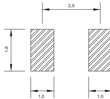
Top View Suggest Layout
