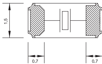
Top View Crystal Connection
